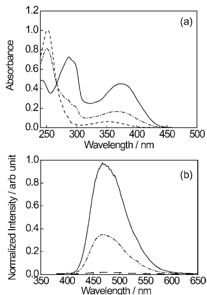
Figure 2. (a) Absorption and (b) fluorescence spectral change of 1 in hexane ( 2.7 \times 10^{-5} mol dm ^{-3} , \lambda_{\text{exc}} = 267 nm) by photoirradiation: 1a (—), 1 in the photostationary state under irradiation with \lambda > 380 -nm light (---), and 1b (---).
